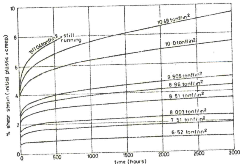
FIG. 6 TORSION CREEP CURVES FOR 0.18 PERCENT CARBON STEEL AT 400^{\circ}\text{C}
