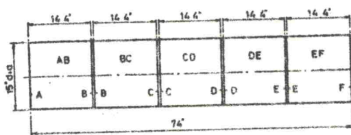
FIG. 5(a) INITIAL CUTTING DIAGRAM
